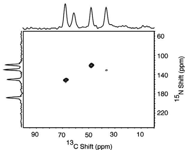
Fig. 10. Two-dimensional ^{15}\text{N}/^{13}\text{C} HETCOR spectrum of the ^{13}\text{C}_\alpha , ^{15}\text{N} labeled single crystal of N -acetyl leucine ( ^{13}\text{C}_\alpha , ^{15}\text{N} NAL) obtained using the pulse sequence in Fig. 1e. Four scans for each of 90 t_1 points were acquired in the indirect dimension with a dwell of 50 \mu\text{s} . The ^1\text{H} decoupling field during the t_1 and t_2 intervals was 50 kHz. The recycle delay used for the experiment was 6 s.
