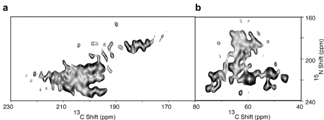
Fig. 11. Two-dimensional ^{15}\text{N}/^{13}\text{C} HETCOR spectrum of the magnetically aligned sample of Pfl bacteriophage with the coat protein labeled with both ^{13}\text{C} and ^{15}\text{N} . The spectrum was acquired at 0^\circ\text{C} . Thirty two scans of 80 complex points were acquired in the indirect dimension with a spectral width of 30 kHz. The recycle delay was 6 s. The data were zero filled to 1K points and multiplied by a sine bell window function in both dimensions prior to double Fourier transformation. The carrier frequency for ^{13}\text{C} irradiation was in the center of the spectrum, between the aliphatic and carbonyl resonance regions, and the double cross-polarization was optimized for both types of resonances.
