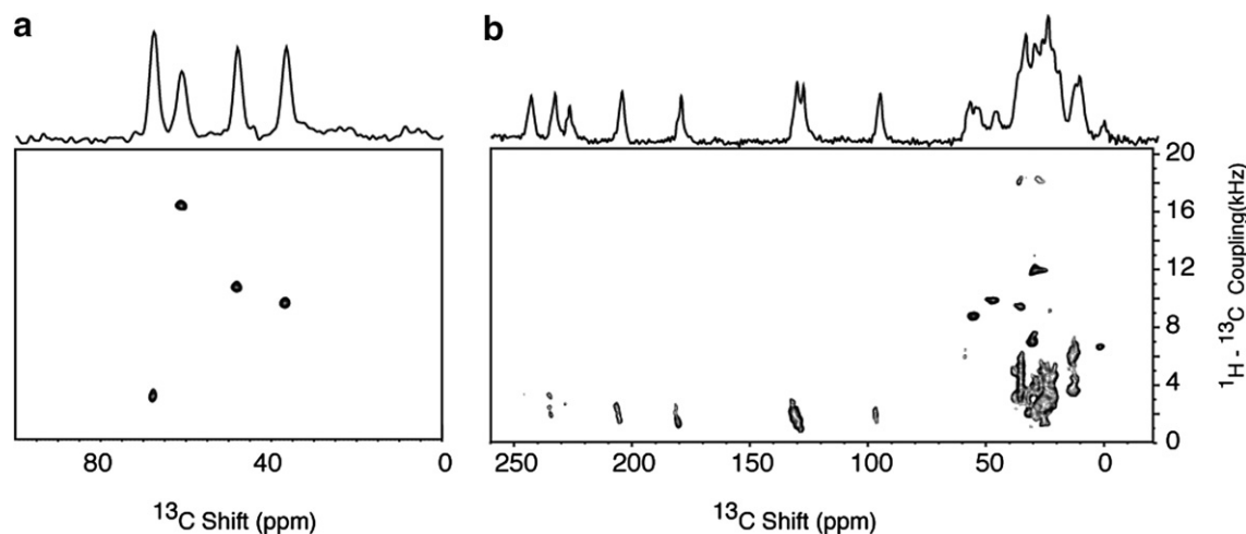
Fig. 3. Two-dimensional ^1\text{H} - ^{13}\text{C} PISEMA spectra obtained using the pulse sequence in Fig. 1a. (a) Spectrum from the ^{13}\text{C}_\alpha , ^{15}\text{N} labeled single crystal of N -acetyl leucine ( ^{13}\text{C}_\alpha , ^{15}\text{N} NAL) obtained with 4 scans for each of 128 t_1 points. (b) Spectrum from the ^{15}\text{N} labeled single crystal of N -acetyl valine (NAV) obtained with 8 scans for each of 128 t_1 points. During the heteronuclear spin exchange period ( t_1 ), the radiofrequency field strength of 55 kHz power level on the ^1\text{H} channel enabled the maximum ^1\text{H} - ^{13}\text{C} dipolar couplings to be observed without aliasing. The recycle delay was 6 s. The two-dimensional data sets were zero filled to 1K data points and multiplied by a sine bell window function in both dimensions before double Fourier transformation.
