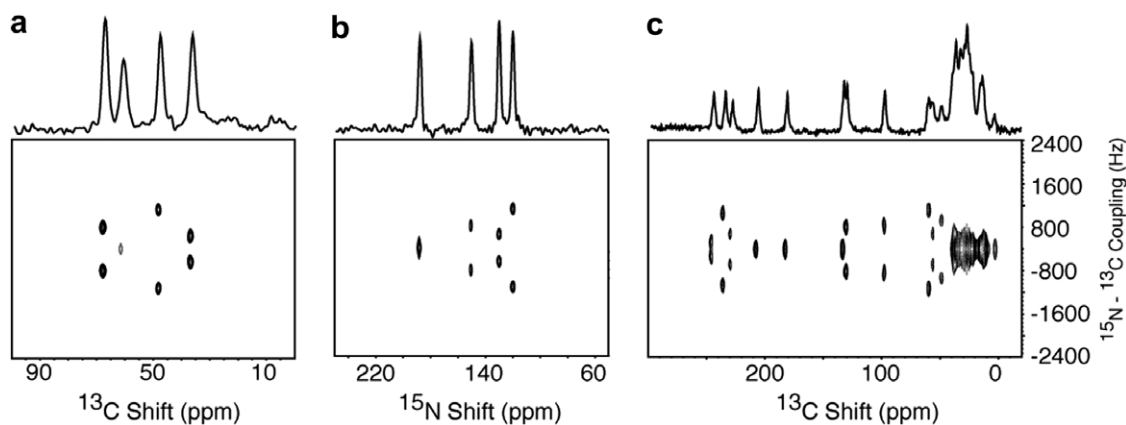
Fig. 8. Two-dimensional ^{13}\text{C} - ^{15}\text{N} SLF spectra obtained using the pulse sequence in Fig. 1b. (a) and (b) are from the ^{13}\text{C}_\alpha , ^{15}\text{N} labeled single crystal of N -acetyl leucine ( ^{13}\text{C}_\alpha , ^{15}\text{N} NAL). (c) Is from the ^{15}\text{N} labeled single crystal of N -acetyl valine (NAV). (a) and (c) ^{13}\text{C} detected. (b) ^{15}\text{N} detected. For spectra a and b, four scans were collected for 48 points in the indirect dimension with 100 \mu\text{s} dwell time and 16 scans were collected for spectrum c.
