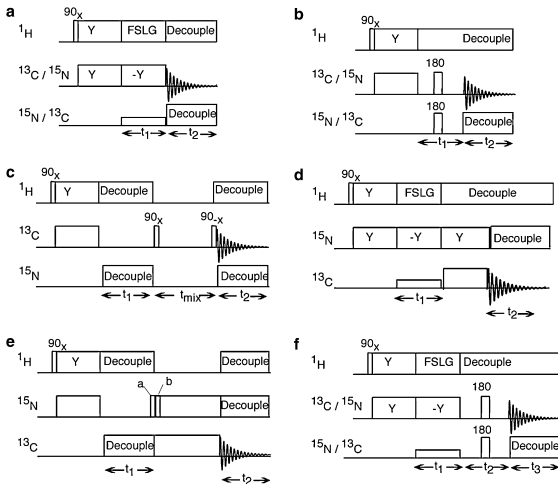
Fig. 1. Timing diagrams for triple-resonance solid-state NMR experiments. (a) Two-dimensional ^1\text{H} - ^{13}\text{C} or ^1\text{H} - ^{15}\text{N} PISEMA. The pulse sequence for the triple resonance version of the PISEMA is same as its double resonance version except that low power irradiation (mismatched to the irradiations in the other two channels) is applied during t_1 period at the resonance frequency of the undetected nucleus. (b) Two-dimensional ^{13}\text{C} - ^{15}\text{N} dipolar coupling measurement. The phase of the 180^\circ pulse is same as for the cross-polarization irradiation. The receiver phase is cycled as (x, -x) and the 90^\circ pulse on the ^1\text{H} channel is phase cycled as (x, -x) . (c) Two-dimensional ^{13}\text{C}/^{13}\text{C} spin exchange. The 90^\circ pulse after the t_1 period is phase incremented by 90^\circ for quadrature detection. (d) Two-dimensional ^1\text{H} - ^{15}\text{N} PISEMA with ^{13}\text{C} detection. (e) Two-dimensional ^{13}\text{C}/^{15}\text{N} HETCOR. (f) Three-dimensional ^1\text{H} - ^{13}\text{C} dipolar coupling/ ^{13}\text{C} - ^{15}\text{N} dipolar coupling/ ^{13}\text{C} chemical shift or ^1\text{H} - ^{15}\text{N} coupling/ ^{13}\text{C} - ^{15}\text{N} dipolar coupling/ ^{15}\text{N} chemical shift correlation.
