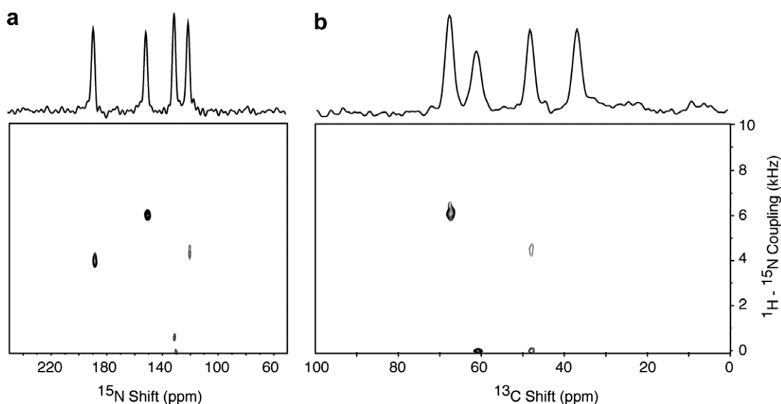
Fig. 6. Two-dimensional ^1\text{H} - ^{15}\text{N} PISEMA spectra of the ^{13}\text{C} , ^{15}\text{N} labeled single crystal of N -acetyl leucine ( ^{13}\text{C} , ^{15}\text{N} NAL). (a) ^{15}\text{N} detected. (b) ^{13}\text{C} detected. Sixteen scans were acquired for each of 128 points in the indirect dimension for spectrum a and 32 scans for spectrum b. The contact time was 1.0 ms during the double cross-polarization from ^{15}\text{N} to ^{13}\text{C} , and the recycle delay was 5 s.
