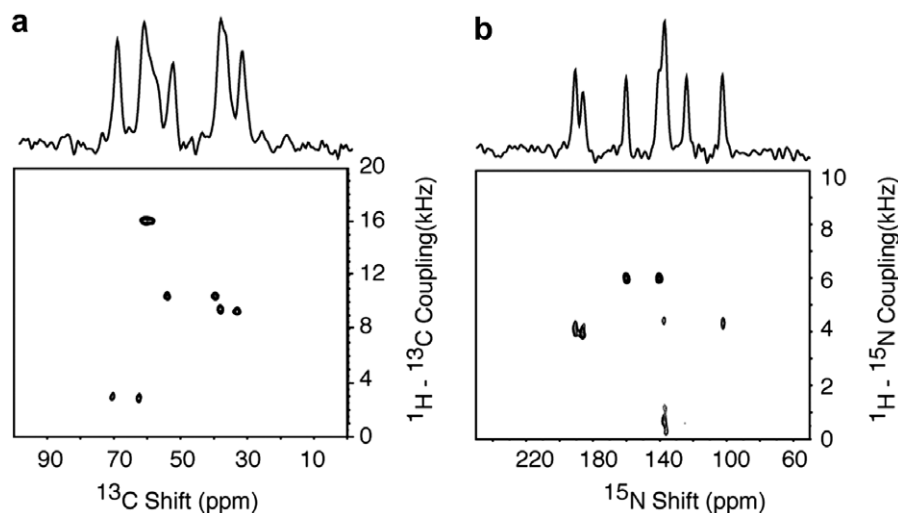
Fig. 9. Two-dimensional PISEMA spectra of the ^{13}\text{C}_\alpha , ^{15}\text{N} labeled single crystal of N -acetyl leucine ( ^{13}\text{C}_\alpha , ^{15}\text{N} NAL). (a) ^1\text{H} - ^{13}\text{C} PISEMA spectrum obtained without ^{15}\text{N} decoupling during acquisition ( t_2 ). (b) ^1\text{H} - ^{15}\text{N} PISEMA spectrum obtained without ^{13}\text{C} decoupling during acquisition ( t_2 ). For the 2D spectrums, 4 scans were added for each t_1 points (128). During spin exchange period, 55 kHz power level on the ^1\text{H} channel were used. The two-dimensional data sets were zero filled to 1K data points and multiplied by sine bell window function before double Fourier transformation. The one-dimensional ^{13}\text{C} (a) and ^{15}\text{N} (b) NMR spectra obtained without decoupling of the unobserved nucleus are aligned along the corresponding two-dimensional spectra.
