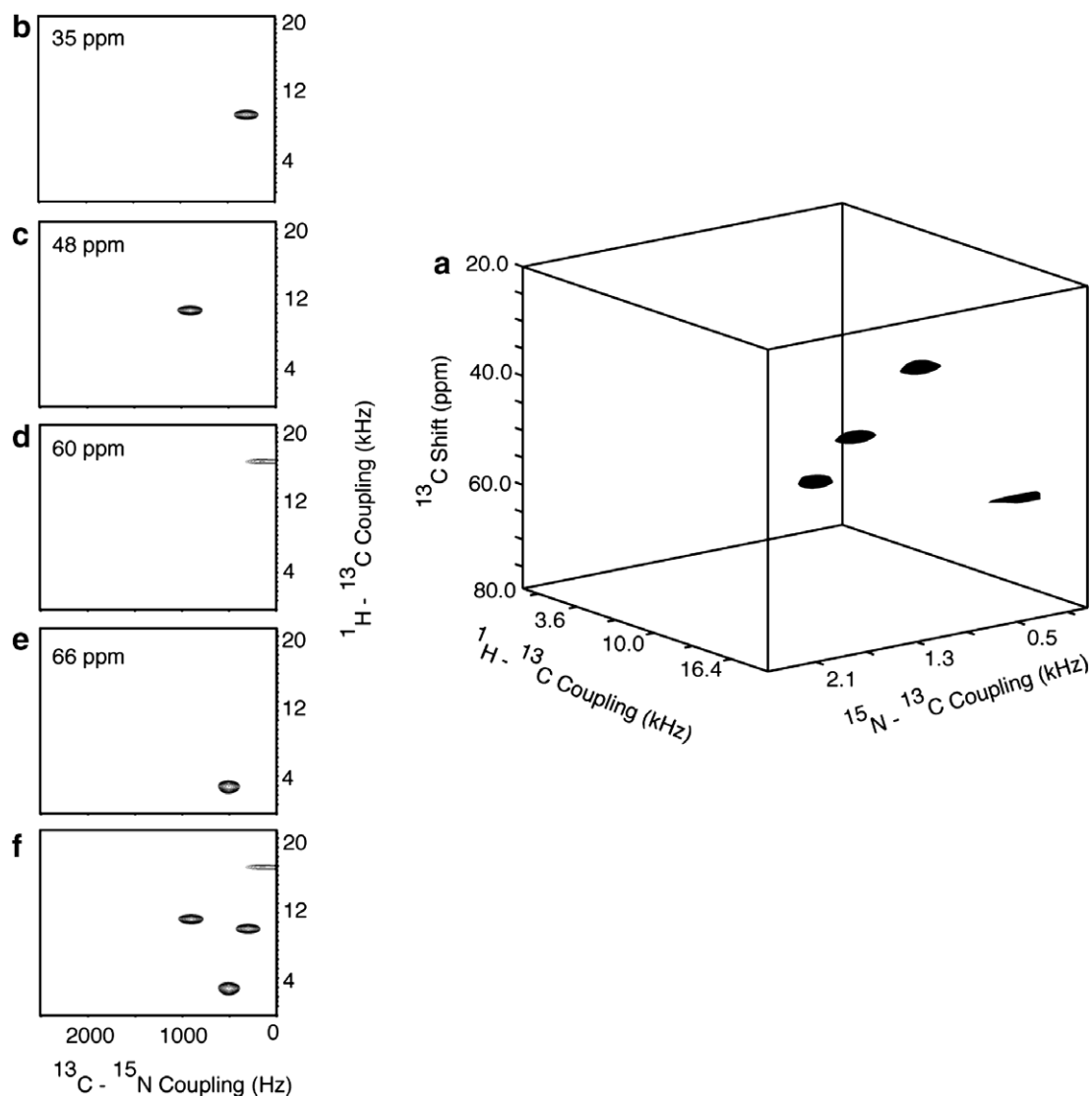
Fig. 12. Results from the three-dimensional experiment diagrammed in Fig. 1f that correlates ^{13}\text{C} chemical shift/ ^1\text{H} - ^{13}\text{C} dipolar coupling/ ^{13}\text{C} - ^{15}\text{N} dipolar coupling frequencies performed on the ^{13}\text{C}_\alpha, ^{15}\text{N} labeled single crystal of N -acetyl leucine ( ^{13}\text{C}_\alpha, ^{15}\text{N} NAL). (a) Three-dimensional cube displaying all four resonances. (b)–(e) Two-dimensional planes at ^{13}\text{C} chemical shift frequencies containing resonance intensity. (f) Two-dimensional projection. 32 points in the ^1\text{H} - ^{13}\text{C} dimensions (spectral width = 40 kHz) and 21 points in the ^{13}\text{C} - ^{15}\text{N} dimensions (spectral width = 5.0 kHz) were acquired with 4 scans.
