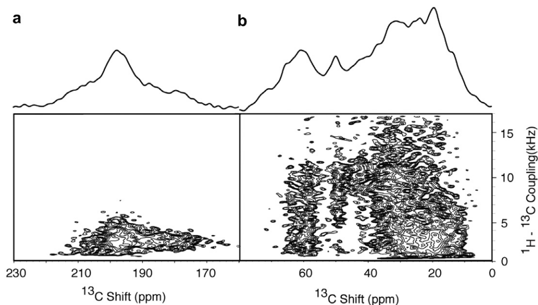
Fig. 5. Two-dimensional ^1\text{H} - ^{13}\text{C} PISEMA spectrum of the structural form of the 46-residue Pfl coat protein in magnetically aligned virus particles where the protein is labeled \sim 20\% randomly with ^{13}\text{C} and \sim 100\% uniformly with ^{15}\text{N} Pfl ( ^{13}\text{C} and ^{15}\text{N} Pfl). (a) Carbonyl and carboxyl carbon resonances. (b) Aliphatic carbon resonances. Thirty two scans were acquired for each of 128 points in the indirect dimension. The recycle delay was 6 s, and the temperature 0^\circ\text{C} . The central ^1\text{H} carrier frequency during t_1 was +2 ppm relative to the water resonance during the PISEMA portion of the pulse sequence. The two-dimensional data set was zero filled to 1K data points and multiplied by a sine bell window function in both dimensions before double Fourier transformation.
