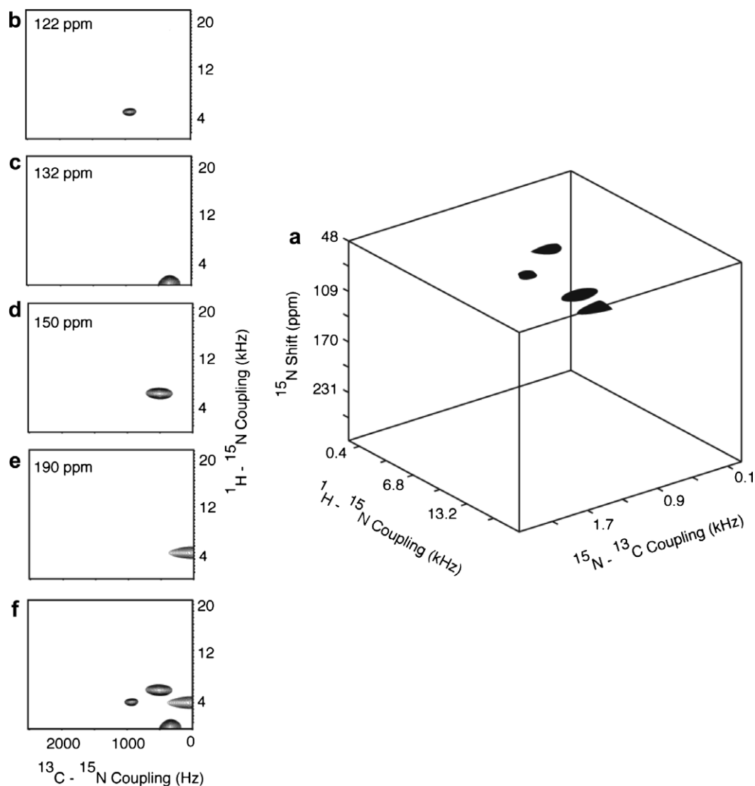
Fig. 13. Results from the three-dimensional experiment diagrammed in Fig. 1f that correlates ^{15}\text{N} chemical shift/ ^1\text{H} - ^{15}\text{N} dipolar coupling/ ^{13}\text{C} - ^{15}\text{N} dipolar coupling frequencies performed on the ^{13}\text{C}_\alpha , ^{15}\text{N} labeled single crystal of N -acetyl leucine ( ^{13}\text{C}_\alpha , ^{15}\text{N} NAL). (a) Three-dimensional cube displaying all four resonances. (b)–(e) Two-dimensional planes at ^{15}\text{N} chemical shift frequencies containing resonance intensity. (f) Two-dimensional projection. 32 points in the ^1\text{H} - ^{15}\text{N} dimensions (spectral width = 40 kHz) and 21 points in the ^{13}\text{C} - ^{15}\text{N} dimensions (spectral width = 5.0 kHz) were acquired with 4 scans.
