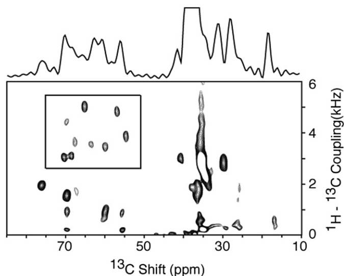
Fig. 4. Two-dimensional ^1\text{H} - ^{13}\text{C} PISEMA spectrum of the membrane-bound form of the 46-residue Pf1 coat protein in magnetically aligned phospholipid bilayers where the protein is labeled with ^{13}\text{C}_\alpha and ^{15}\text{N} at all valine, leucine and isoleucine residues ( ^{13}\text{C}_\alpha , ^{15}\text{N} VLI Pf1). The spectrum was obtained using the pulse sequence in Fig. 1a. All of the signals in the box are from ^1\text{H} - ^{13}\text{C}_\alpha dipolar couplings. Nearly all of the other intensity observed in the spectrum is from the natural abundance signals from the phospholipids in the sample. Ninety six scans were acquired for each of 128 points in the indirect dimension. The recycle delay was 5 s and the temperature 40 °C. The two-dimensional data set was zero filled to 1K data points and multiplied by a sine bell window function in both dimensions before double Fourier transformation.
